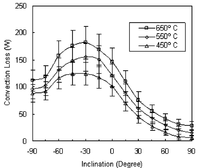
Fig. 7 Convection heat loss from a fully open cylindrical cavity
