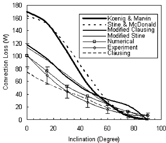
Fig. 12 Comparison of natural convection heat loss for T_c = 445 deg C and cavity fully open
