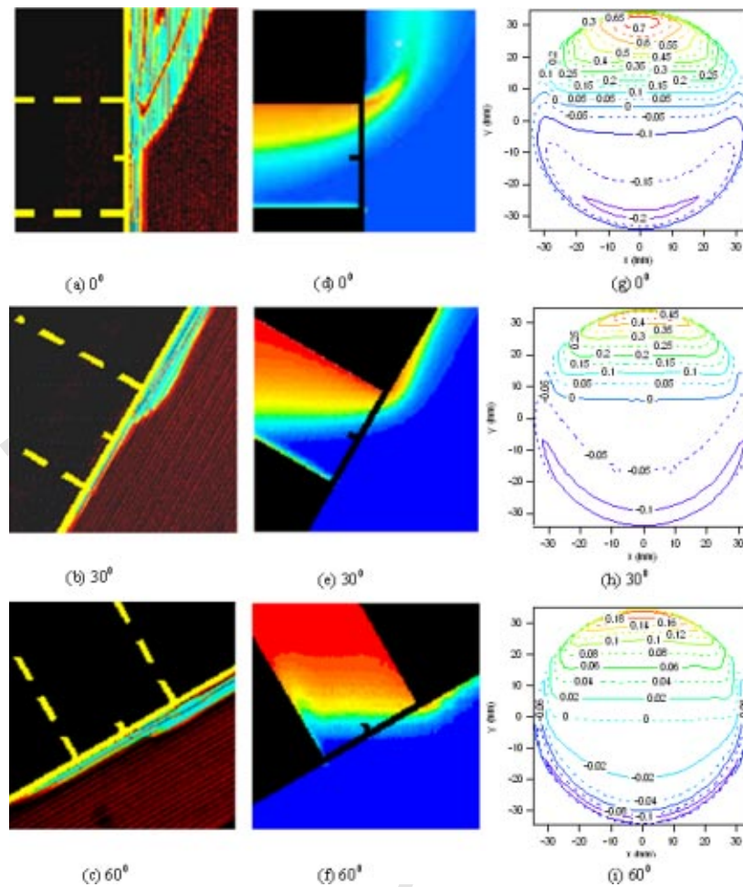
Fig. 11 Aperture region flow images for T_c=445 deg C and fully open cavity: (a)-(c) Schlieren images, (d)-(f) numerical temperature contour plots, (g)-(i) aperture normal velocity profiles
