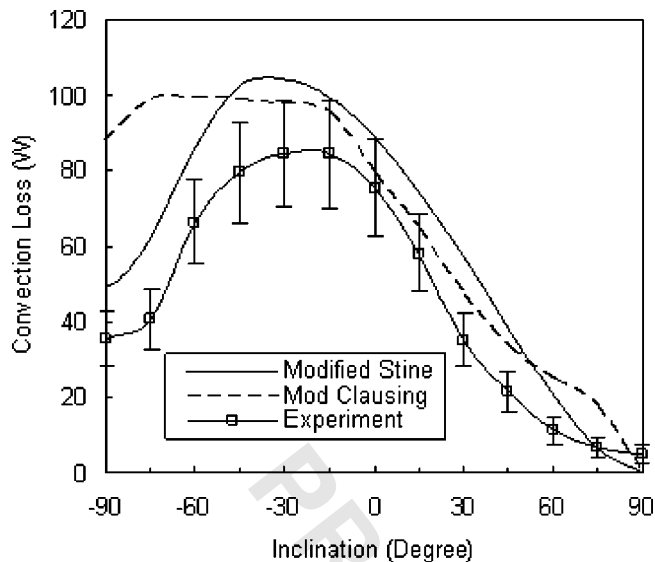
Fig. 14 Comparison of natural convection heat with T_c = 445 deg C and R_{exp} = 0.75
