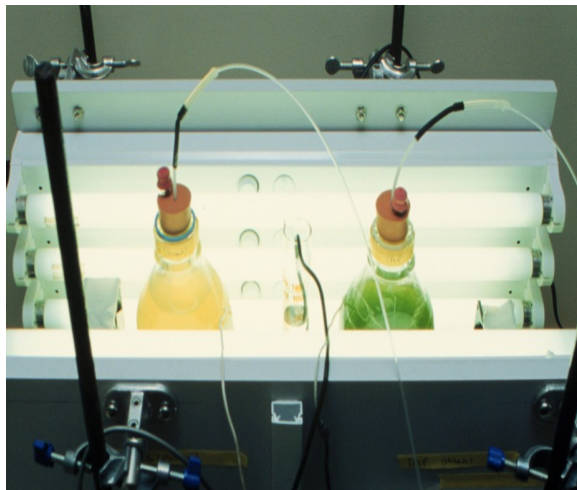
Figure 2. 1 L bottle bioreactor experimental set-up for H 2 production using a sulphur starvation treatment, showing tubing for gas collection (ending inside an underwater inverted graduated cylinder). Two physiological treatments are shown.
