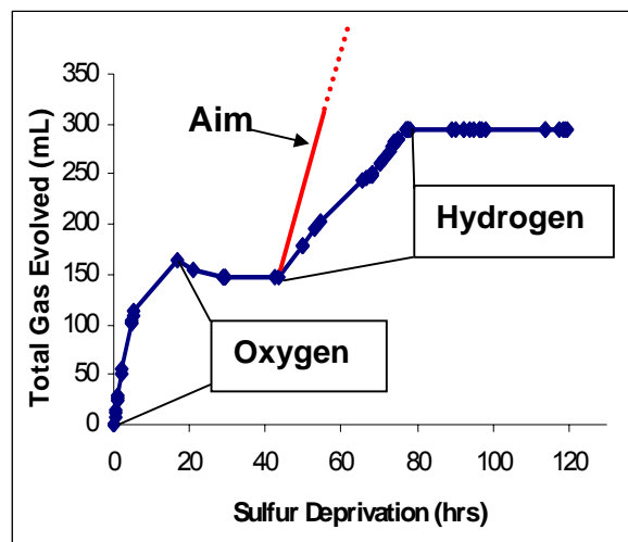
Figure 3. Total gas evolution after sulphur starvation showing the first O 2 evolution phase and the H 2 production phase. The experiment is with a 1L bioreactor as in Figure 2. Gases are identified by gas chromatography.
