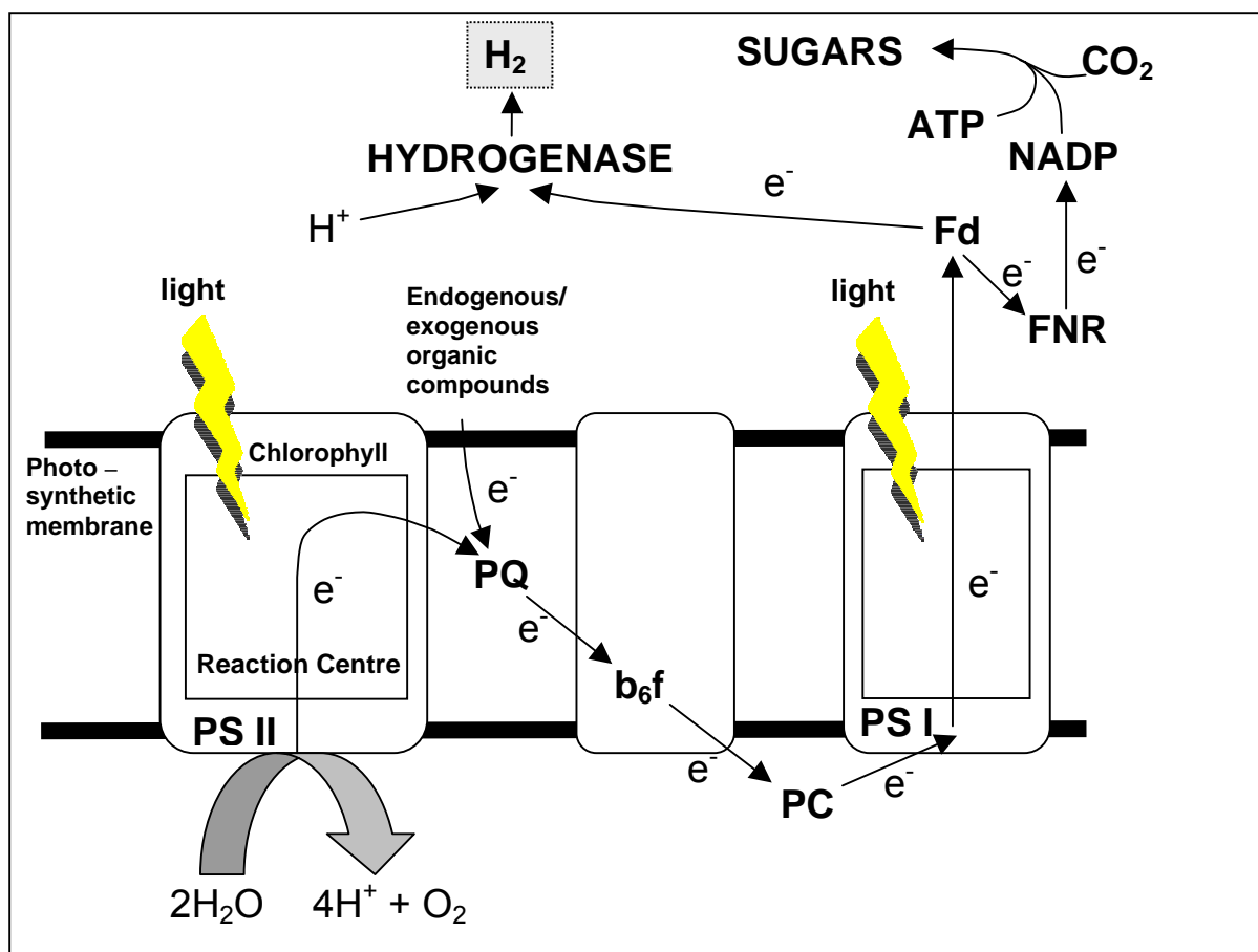
Figure 1. Photosynthetic electron transfer in the chloroplast of the unicellular green alga Chlamydomonas reinhardtii and the alternative H 2 production pathway. PS I and PS II are Photosystems I and II, respectively. PQ, PC, Fd and NADP (plastoquinone, plastocyanin, ferredoxin, and nicotinamide-adenosine-dinucleotide-phosphate, respectively) are electron carriers. b 6 f (cytochrome b 6 f complex), FNR (ferredoxin-NADP reductase), and hydrogenase are redox enzymes. ATP (adenosine triphosphate) is a biochemical high-energy intermediate. In normal conditions a linear electron transfer is established that maintains CO 2 fixation for the synthesis of sugars. In the absence of O 2 (see text for conditions) the photosynthetic electron transport is diverted at the level of Fd towards the synthesis of H 2 , which is evolved as a by-product.
