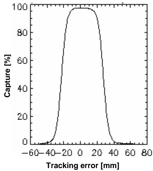
Figure 3.2 Capture vs tracking error at the target plane
