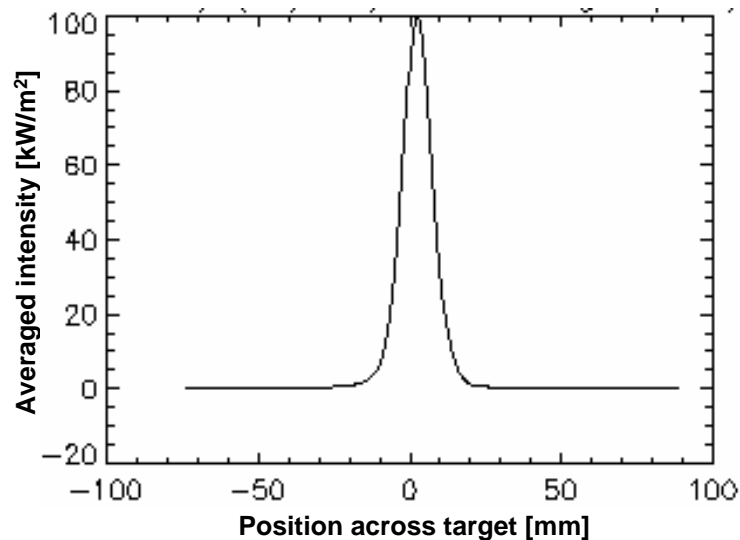
Figure 3.3 Averaged intensity vs position across target
