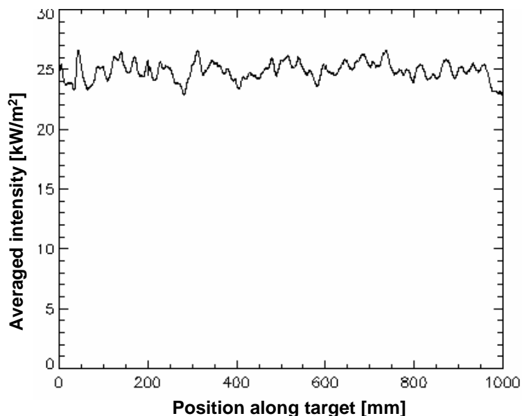
Figure 3.4 Averaged intensity vs position along target for a 50mm receiver width
