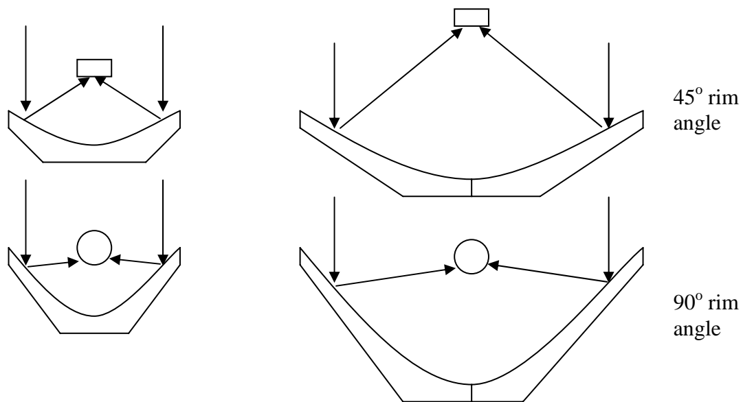
Figure 2.3 Possible trough mirror configurations based around single or double use of the ANU mirror panel type.
