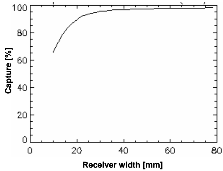
Figure 3.1 Capture vs receiver width
